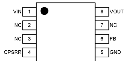
8-Pin MSOP MIC5281YMM
