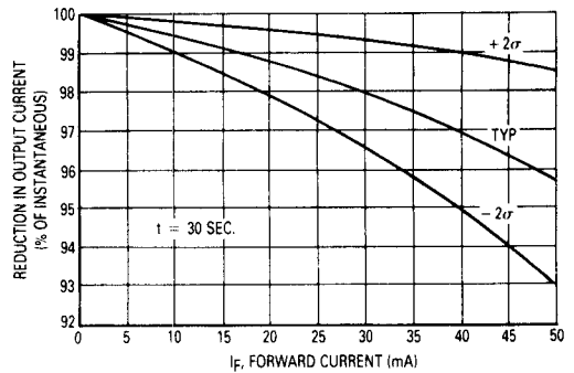
Figure 6. Reduction in Output Current Heating versus Forward Current
