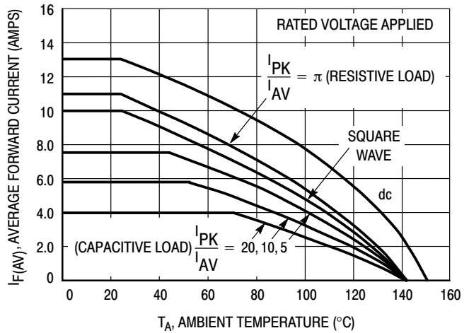
Figure 6. Current Derating, R_{\theta JA} = 16^{\circ}C/W
