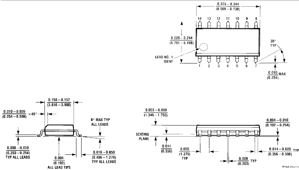
14-Lead Small Outline Molded Package (M) Order Number DM74LS10M NS Package Number M14A
