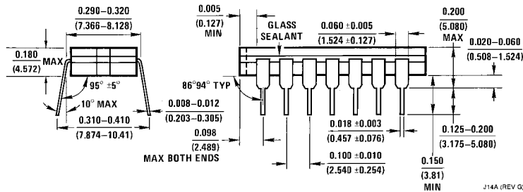
14-Lead Ceramic Dual-In-Line Package (J) Order Number 54LS10DMQB or DM54LS10J NS Package Number J14A
