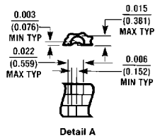
Ceramic Leadless Chip Carrier Package (E) Order Number 54LS10LMQB NS Package Number E20A
