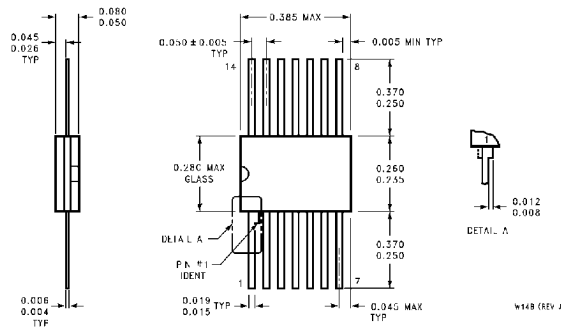
14-Lead Ceramic Flat Package (W) Order Number 54LS10FMQB or DM54LS10W NS Package Number W14B
