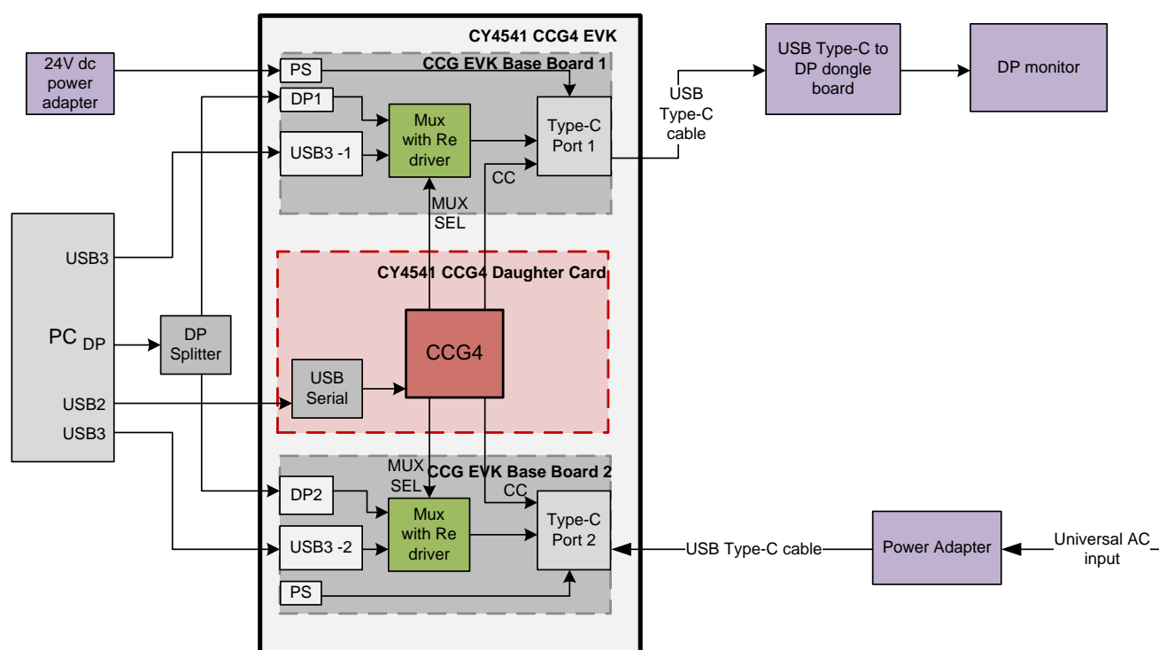
Figure 7. CY4541 EZ-PD CCG4 EVK System-level Block Diagram
