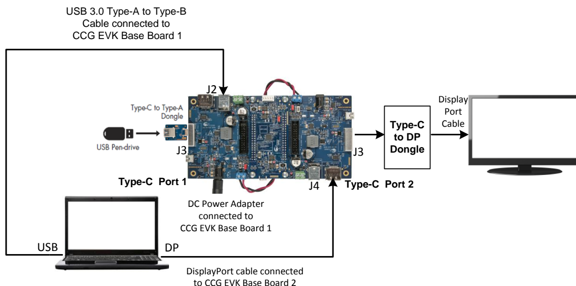
Figure 32. Setup of the DisplayPort Demo
