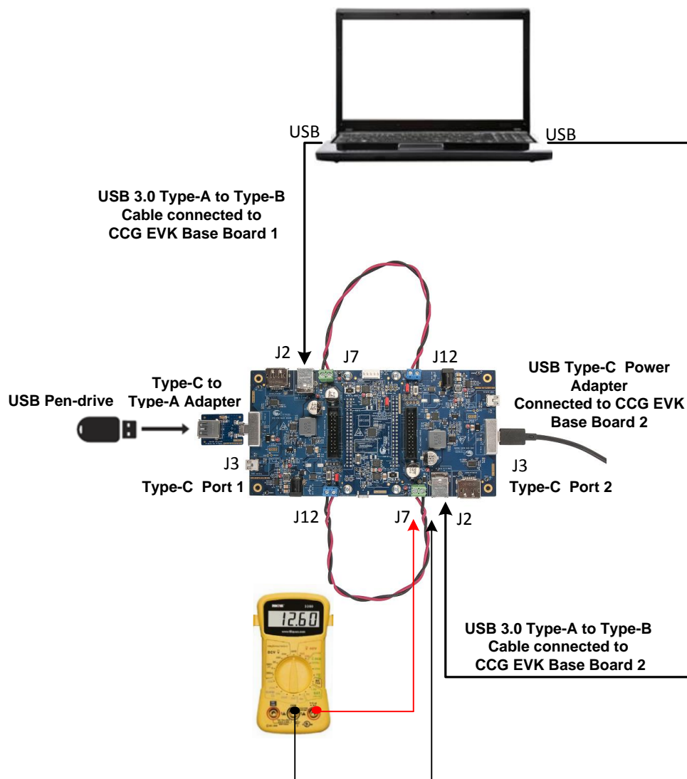
Figure 31. Setup of DRP and Dead Battery Charging Demo (Example 2)
