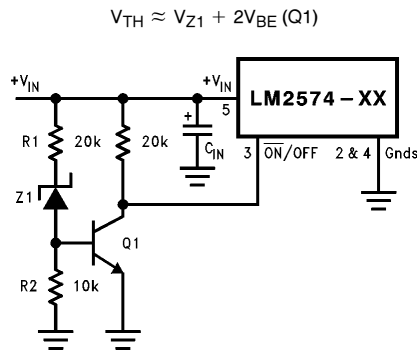
FIGURE 13. Undervoltage Lockout for Buck Circuit
