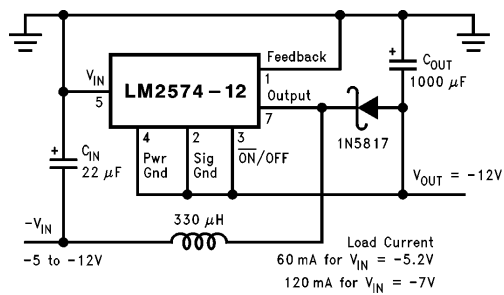
FIGURE 12. Negative Boost
