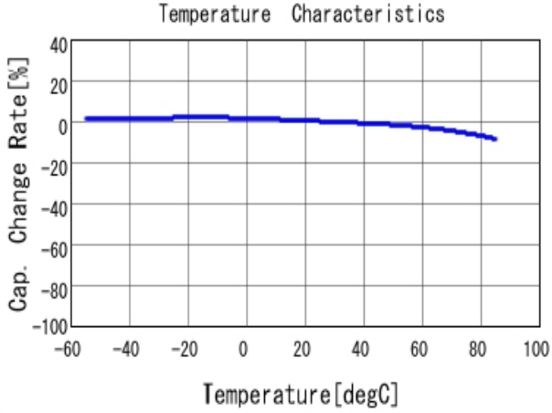
■ GRM219R6YA475MA73 C-Temp. capchange, DC0.0V, AC1.0V rm
