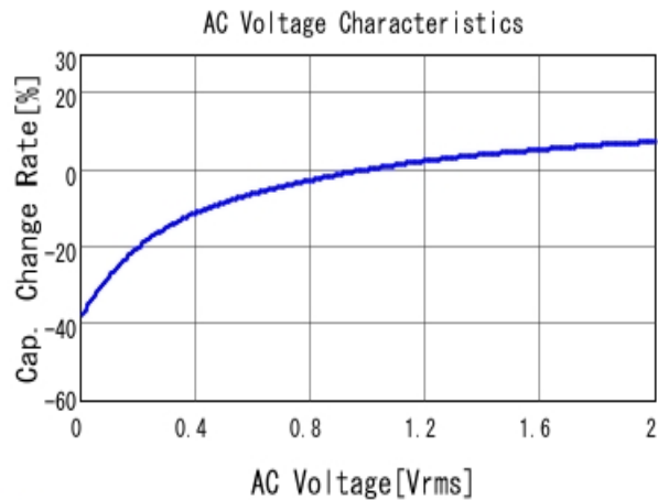
■ GRM219R6YA475MA73 C-AC Voltage capchange, DCOV, 25.0d
