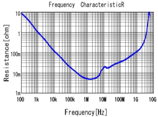
■ GRM219R6YA475MA73 R DCOV, 25degC
