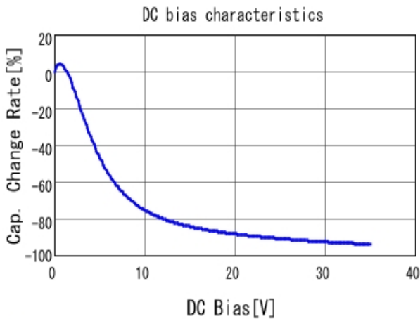
■ GRM219R6YA475MA73 C-DC bias capchange, 25.0degC, AC1.
