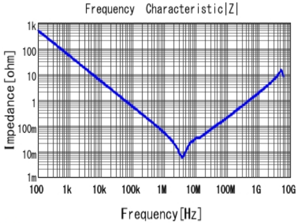
■ GRM219R6YA475MA73 |Z| DCOV, 25degC
