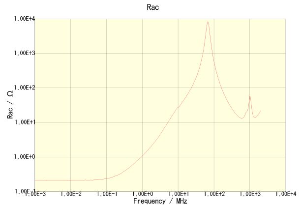
NLCV32T-4R7M-PF
