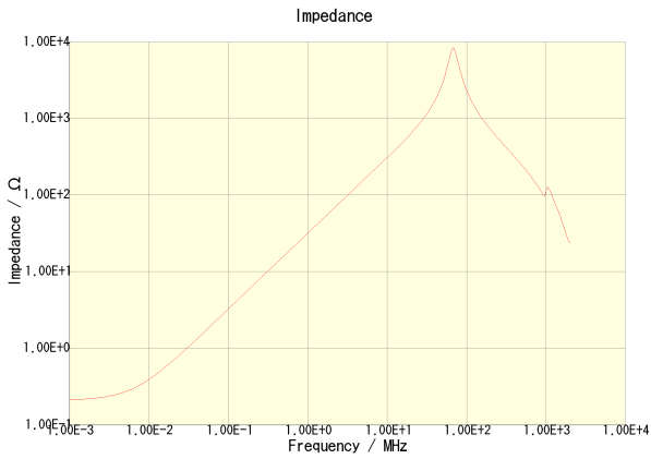
NLCV32T-4R7M-PF
