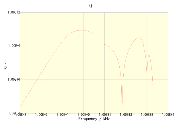
NLCV32T-4R7M-PF
