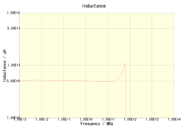
NLCV32T-4R7M-PF
