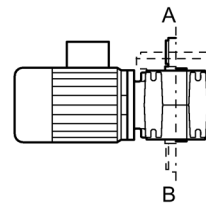
Figure 10-4 Type of construction options for S sizes 08, 18, 28
